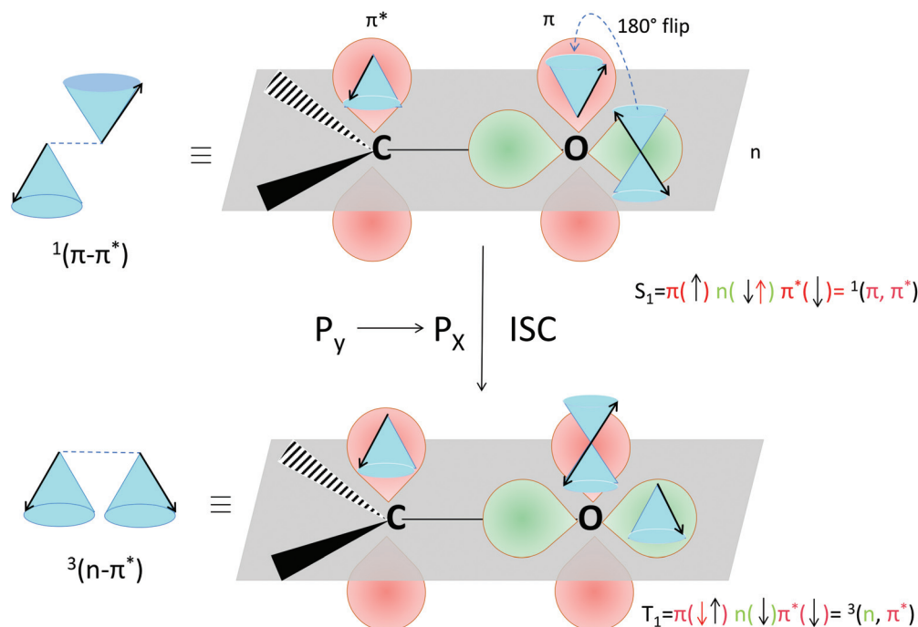
Fig. 14 Visualization of the selection rules for spin–orbit coupling for a carbonyl compound. For a 1(\pi-\pi^*) singlet excited state (top), the transition between the orthogonal doubly occupied n orbital (green) and \pi orbital (red, single occupation) provides the spin–orbit coupling to enable the electron spin flip and produce the 3(n-\pi^*) triplet excited state (bottom). We use the rotating frame vector representation and the selection rules for triplet state formation of a 1(\pi-\pi^*) singlet into a 3(n-\pi^*) triplet (adapted from ref. 67). It is a qualitative orbital description of the basis for allowed intersystem crossing. The red arrow in the two electron configurations depicts the flipping electron. A magnetic field is present in the z direction, for the purpose of simple spin representation.
