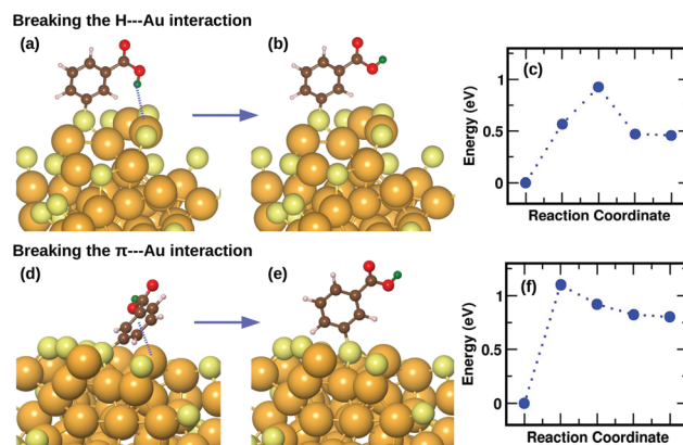
Fig. 5 (a) The optimized structure of \text{Au}_{68}(\text{m-MBA})_{32} highlighting a COOH...Au interaction. (b) The ligand in (a) is modified such that the carboxylic H is pointed away from the Au core breaking the interaction. (d) The optimized structure of \text{Au}_{68}(\text{m-MBA})_{32} highlighting a \pi ...Au interaction, (e) the structure with the ligand in (d) modified such that it stands upright breaking the interaction. (c) and (f) show the energy profiles as obtained from CI-NEB calculations for the minimum energy pathway from structure (a) to (b), and (d) to (e), respectively. Au, S, C, O, phenyl H and carboxylic H are shown in golden, pale yellow, brown, red, white and green colors, respectively. All the ligands were included in the calculation but the other ligands are not shown for clarity.
