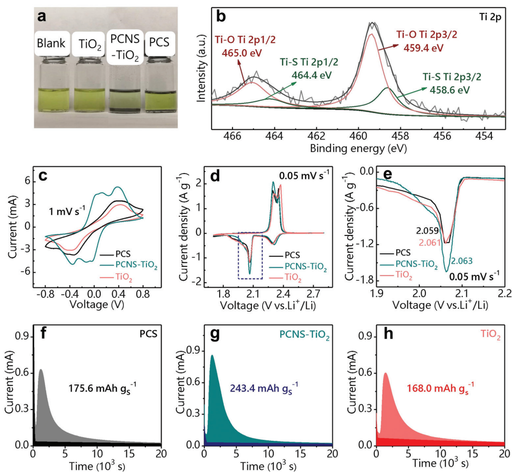
Fig. 3 (a) Li 2 S 6 adsorption test of different samples with the same weight. (b) Ti 2p spectrum of PCNS-TiO 2 after the Li 2 S 6 adsorption test. (c) CV profiles of symmetrical cells with the PCS, PCNS-TiO 2 and TiO 2 at a scanning rate of 1 mV s -1 . CV profiles of Li-S batteries with PCS/S, PCNS-TiO 2 /S and TiO 2 /S as cathodes at a scan rate of 0.05 mV s -1 over a voltage range of 1.7 to 2.8 V (d) and the magnification of the cathodic peak ranging from 1.9 to 2.2 V (e). (f–h) Potentiostatic discharge curves of the Li 2 S deposition measurement. The light-colored area suggests the precipitation of Li 2 S, while the dark-colored area indicates the reduction of Li 2 S 8 /Li 2 S 6 .
