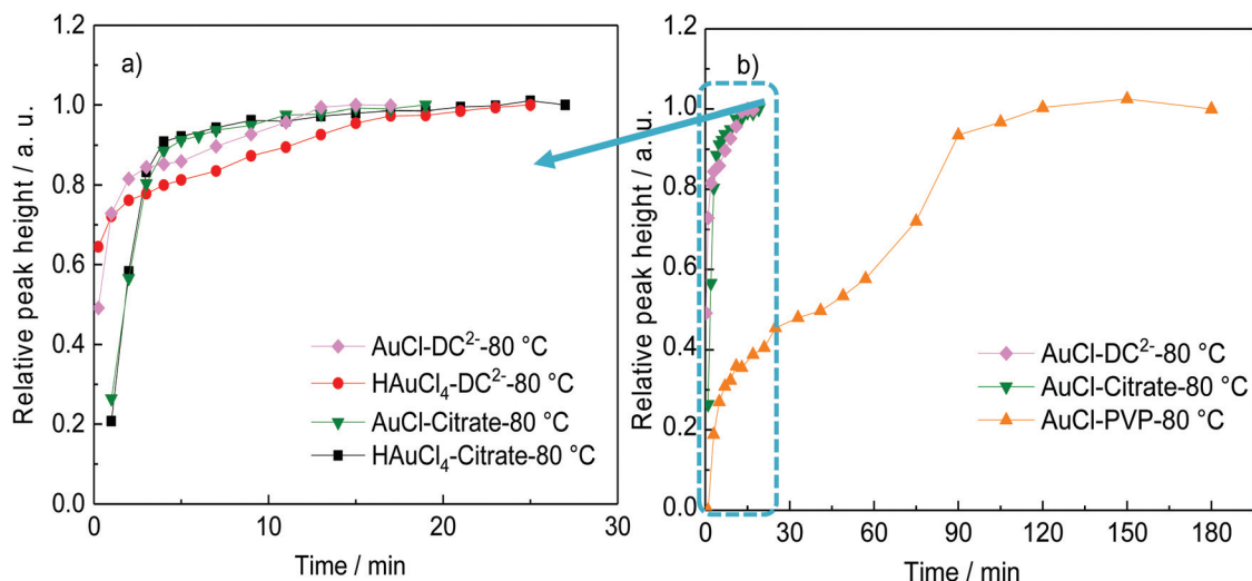
Fig. 4 Comparison of the rate of formation of gold nanoparticles (shown by the relative height of the absorption peak) (a) using different gold precursors and reducing agents at 80 °C. Conditions: [HAuCl 4 ]: 0.25 mM, [AuCl]: 0.25 mM, [sodium citrate]: 2.5 mM, [DC 2- ]: 2.5 mM, pH: 4.8–4.9. Original data are shown in Fig. S3.† (b) By the reduction or the disproportionation reaction of AuCl with DC 2- or sodium citrate as a reducing agent (same with (a)), or PVP as stabilizer in the absence of sodium citrate and DC 2- . Conditions: [AuCl]: 0.25 mM, [PVP monomer]: 5 mM, pH: 4.8, 80 °C.
