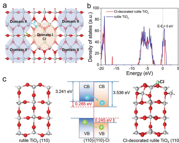
Fig. 1 (a) Scheme of the surface domain heterojunction (SDH), (b) total density of states (TDOSs) of the rutile TiO 2 (110) face with and without Cl decoration, and (c) atomic structures and the band diagram of SDH.
