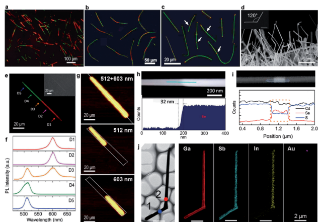
Fig. 4 Axial hetero-nanowires. Real-color optical photograph of (a) dispersed dual-segment CdS–CdSe nanowires, dispersed tri-segment CdS–CdSe nanowires with (b) long and (c) short red-emitting CdS segments in the middle, respectively. (d) SEM of as-grown GaSb–GaInSb nanowires. (e) Real-color optical photograph, (f) spatially resolved PL spectra, and (g) PL peak intensity mapping of a single dual-segment nanowire. (h) HAADF STEM image and line scanning profile of Se along the nanowire length. (i) EDS line profiles of Cd, Se and S across a single tri-segment hetero-nanowire with a short CdS segment in the middle. (j) 2D elemental mapping of GaSb–GaInSb nanowires. (a, e–h) Reproduced with permission. 73 Copyright 2016, American Chemical Society. (b, c and i) Reproduced with permission. 50 Copyright 2017, Elsevier B.V. (d and j) Reproduced with permission. 47 Copyright 2014, American Chemical Society.
