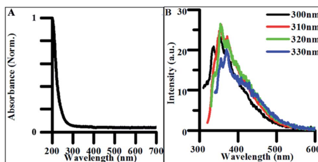
Fig. 3 (A) Normalized absorbance spectrum of undoped CDs synthesized for 4 h. (B) Excitation-independent emission spectra for undoped CDs synthesized for 4 h.
