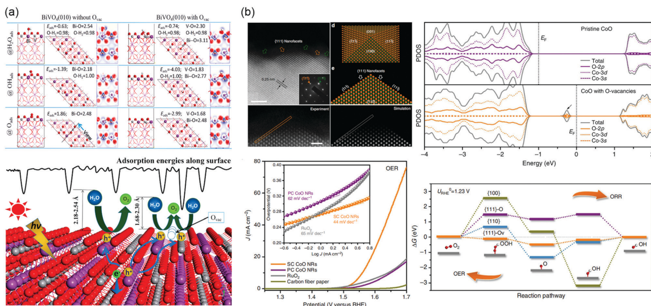
Fig. 10 (a) Top: Adsorption structures, energies and electron density difference of H_2O_{ads} , OH_{ads} and O_{ads} involved in a water splitting process on BiVO_4 (010) facet with V_{Ovac} . Bottom: Schematic picture of the PEC water splitting process on BiVO_4 (010) facet with or without V_{Ovac} . Adsorption energy along surface is illustrated. Reproduced with permission. 256 Copyright 2017 American Chemical Society. (b) Upper left: High-resolution HAADF-STEM image taken from the outermost surface of a single SC CoO NR revealing the exposed {111} nanofacets, with inset showing the corresponding selected area electron diffraction pattern taken from [110] zone axis. Scale bar is 2 nm. Experimental and simulated HAADF-STEM images of the pyramidal structure, respectively. Scale bar is 1 nm. Atomic model of a nanopyramid enclosed with {100} and {111} facets, and the projection of this pyramidal structure along [110] zone axis. Bottom left: OER LSVs of SC, PC CoO NRs and commercial RuO_2 catalysts directly deposited on CFP in O_2 -saturated 1 M KOH solution at scan rate of 0.5\text{ mV s}^{-1} without iR correction, with the corresponding OER Tafel plots shown in inset. Upper right: The calculated ORR/OER free energy diagram at the equilibrium potential on different facets. Bottom right: The projected density of states (PDOS) on pristine CoO and CoO with O-vacancies. Reproduced with permission. 264 Copyright 2016 Springer Nature.
