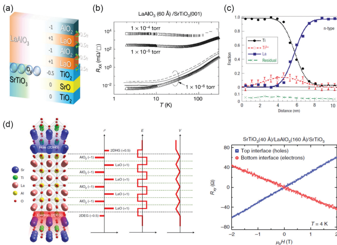
Fig. 6 (a) Sketch of two mechanisms, polar discontinuity and oxygen vacancies, for inducing mobile electrons at the \text{LaAlO}_3/\text{SrTiO}_3 interface. Reproduced with permission. 3,378 Copyright 2018 Wiley-VCH and Copyright 2013 American Physical Society. (b) Temperature-dependent sheet resistance R_{xx} for the interface between \text{LaAlO}_3 and \text{SrTiO}_3 . Reproduced with permission. 135 Copyright 2004 Springer Nature. (c) \text{AlO}_2/\text{LaO}/\text{TiO}_2 interface showing the fractions of elemental Ti and La from the Ti-L and La-M edges, as well as the \text{Ti}^{3+} fraction determined from a least-squares fit to the Ti-L edge from \text{Ti}^{3+} and \text{Ti}^{4+} reference spectra. There is excess \text{Ti}^{3+} on the substrate side of the interface. Reproduced with permission. 149 Copyright 2006 Springer Nature. (d) Left: Schematics that depict the electronic reconstruction across the oxide heterostructure. Right: Hall resistance R_{xy} versus magnetic field \mu_0 H for the top and bottom interfaces at 4 K. The top interface clearly shows a positive slope, which indicates p-type conductivity, whereas the bottom interface shows a negative slope, which indicates n-type conductivity. Reproduced with permission. 150 Copyright 2018 Springer Nature.
