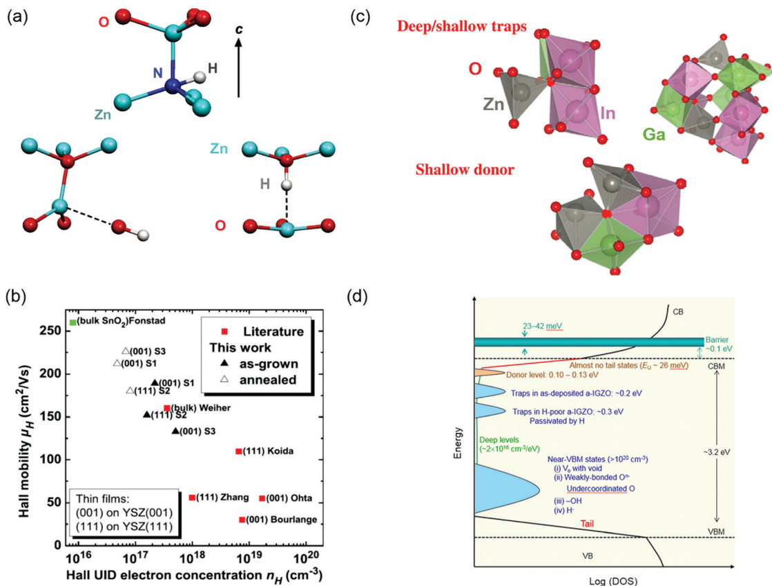
Fig. 12 (a) Structural diagram hydrogen defects in ZnO: Interstitial hydrogen donors (bottom) with antibonding (bottom left) and bond-centered (bottom right) configurations, and nitrogen–hydrogen complex (top). The dashed lines indicate broken Zn–O bonds. Reproduced with permission. 302,328 Copyright 2009 American Institute of Physics and Copyright 2007 American Physical Society. (b) Hall mobility and Hall electron concentration in unintentionally doped (UID), In 2 O 3 thin films and bulk samples. The decreasing electron concentration with simultaneous increase of mobility after annealing in oxygen-containing atmosphere is shown. Reproduced with permission. 299 Copyright 2010 American Institute of Physics. (c) Local coordination structures of some oxygen deficiencies in IGZO. The red spheres represent O ions, green spheres are Ga, grey spheres are Zn and pink spheres are In atoms. The red spheres indicated by the arrows are oxygen vacancy sites. ‘Corner-shared’, ‘Free-space’ and ‘Edge/Face-shared’ notation describes the structures around these oxygen vacancy sites. Reproduced with permission. 298 Copyright 2010 Institute of Physics. (d) Summary of known electronic structure of a-IGZO with subgap defects. Reproduced with permission. 304 Copyright 2019 Wiley-VCH.
