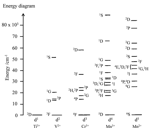
Fig. 3 Energy diagram of the atomic terms computed for the free ions' d^n configurations assuming B = 1000 cm -1 and C/B = 4.7 for the Racah parameters (the diagrams for d^{10-n} are the same as those for d^n ). 5
