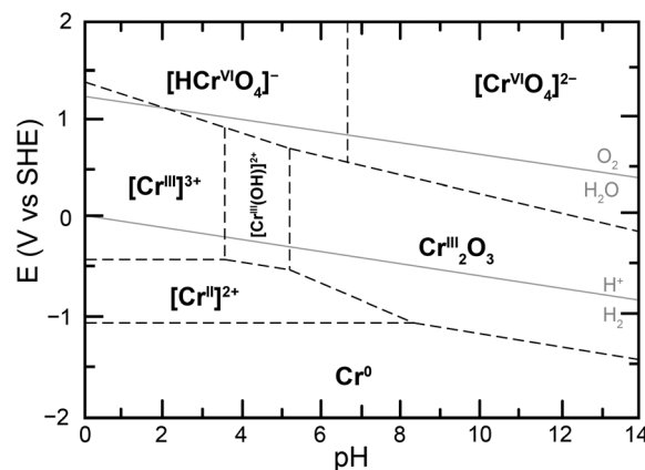
Fig. 2 Proposed calculated Pourbaix diagram for chromium at 10 -6 M total dissolved chromium and 25 °C, adapted from ref. 20.
