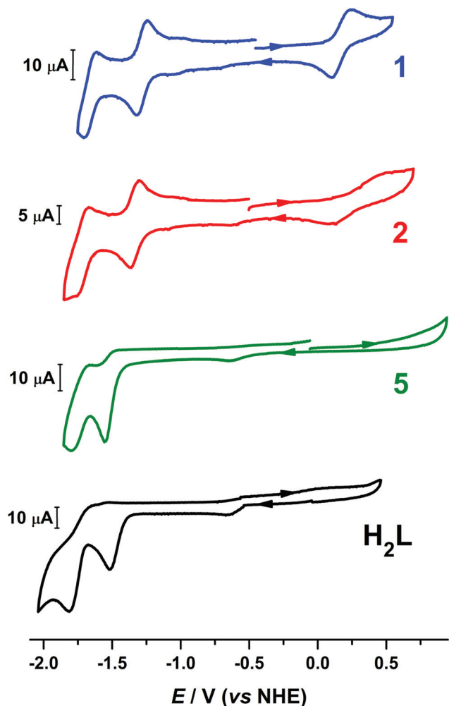
Fig. 4 Comparison of the voltammograms of 1 , 2 , [\text{Zn}_2(\mu\text{-L})_2] ( 5 ) and \text{H}_2\text{L} in 95 : 5 (v/v) DMF/ \text{H}_2\text{O} solution containing 0.1 M [\text{N}(\text{n-Bu})_4]\text{ClO}_4 as supporting electrolyte at scan rate of 100 \text{ mV s}^{-1} .
