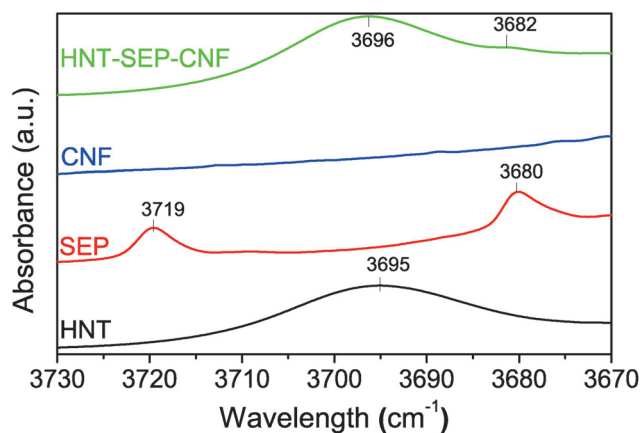
Fig. 5 FTIR spectra of the HNT, SEP, CNF and HNT-SEP-CNF hybrid nanopaper (3730–3670 \text{cm}^{-1} range). The complete spectra are provided in Fig. S3.†
