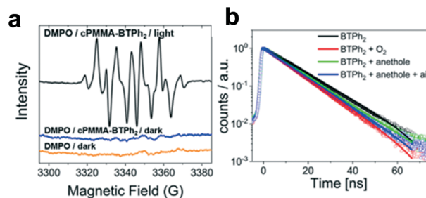
Fig. 3 (a) EPR spectra of DMPO–O 2 •- adducts with cPMMA-BTPPh 2 as the photocatalyst in darkness and under blue light irradiation ( \lambda = 460 nm, 1.2 W cm -2 ). (b) Time-resolved photoluminescence spectra of BTPPh 2 under N 2 (black), under O 2 (red), and with trans -anethole under N 2 (green) and in air (blue) with 20 mg mL -1 of BTPPh 2 and 2 mM trans -anethole in acetonitrile.
