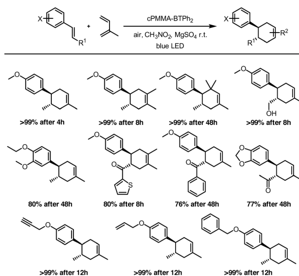
Fig. 4 Scope of the photocatalytic Diels–Alder reaction using cPMMA-BTPPh 2 as the photocatalyst. The reactions were irradiated with a blue LED lamp (460 nm, 0.16 W cm -2 ).
