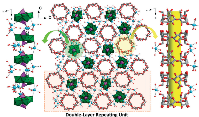
Fig. 2 Combined polyhedral/ball-and-stick representation of Na-PMo- \alpha -CD . Color code: \text{MoO}_6 , green octahedra; \text{PO}_4 pink tetrahedra; Na, turquoise; O, red; C, gray.
