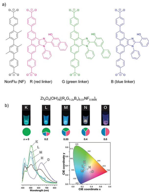
Fig. 4 (a) Solid solution formation with different RGB chromophore linkers in the UiO-type MOF [Zr_6O_4(OH)_4(NonFlu)_6] . (b) Luminescence images (top), spectra (bottom left) and CIE chromaticity coordinates (bottom right) (under \lambda_{ex} = 365 nm irradiation) of the one to three-component RGB MOFs (with chromophore composition indicated in the cake diagrams below the luminescence images). Reproduced from ref. 61 with permission from the American Chemical Society, copyright 2019.
