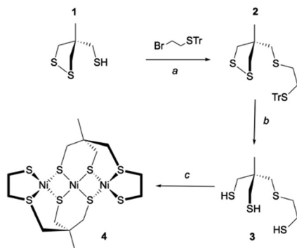
Scheme 1 Synthetic route for the nickel complex 4 . Conditions: (a) NaH, THF, 0 °C to RT, overnight, 66%; (b) CF 3 COOH (excess), Et 3 SiH (3 eq.), CH 2 Cl 2 , RT overnight, 81%; (c) [Ni(CH 3 CN) 6 ](BF 4 ) 2 , K 2 CO 3 (3 eq.), CH 3 CN, RT, 2 h.
