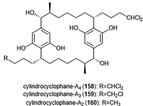
Chart 39 The cylindrocyclophanes A2 and A4 are depicted.
