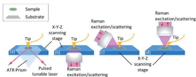
Fig. 3 Working principle and system geometries of AFM and complementary chemical analysis methods. (a) AFM-IR, (b) AFM-TERS bottom-illumination, (c) AFM-TERS side-illumination, and (d) AFM-TERS top-illumination.
