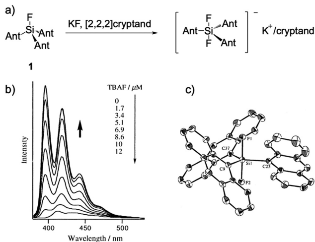
Fig. 1 (a) Reaction scheme of F^- sensor 1 . (b) Fluorescence titration of 1 with TBAF in THF, [ 1 ] = 0.2 \mu\text{M} . (c) Single crystal structure of the complex, K^+/[2.2.2] cryptand is omitted for clarity. Reproduced with permission from ref. 14. Copyright 2000, American Chemical Society.
