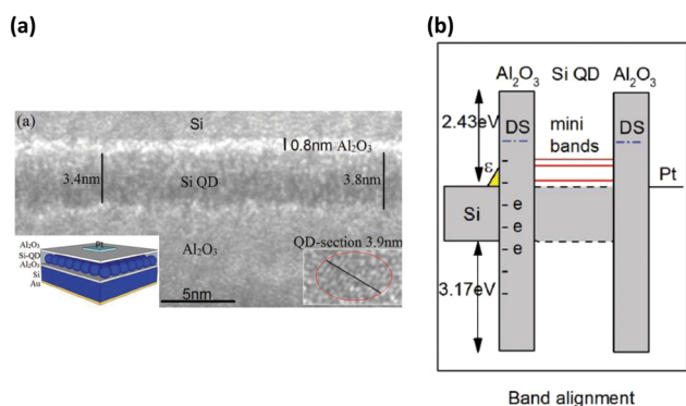
Fig. 2 TEM cross-section and sketch of an ESC based on silicon QDs (a). The QDs are sandwiched between thin layers of Al 2 O 3 to form a double barrier resonant tunnelling structure. The sketch in (b) shows the involved energy levels with the discrete levels of Si QDs within the barrier. 26 Copyright 2017, published by Wiley-VCH.
