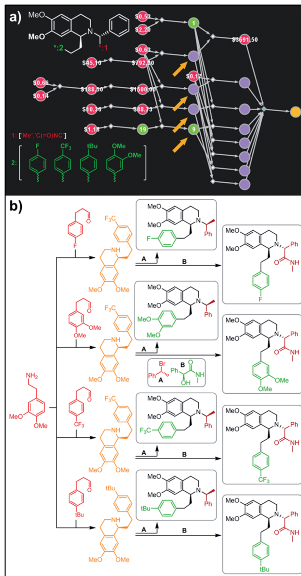
Fig. 6 Retrosynthetic search to synthesize all members of a library of analogues of Almorexant. (a) Markush structure representing proposed library (white inset, top-left) and graph representation of the top-scoring solution. Chemical details are shown in panel (b). Note that several substances (marked with arrows and colored orange in panel (b)) are common intermediates in multiple pathways while the entire library is prepared from single phenylethylamine. For raw Chematica output and further details, see Fig. S8.† Node coloring scheme is as in Fig. 4.
