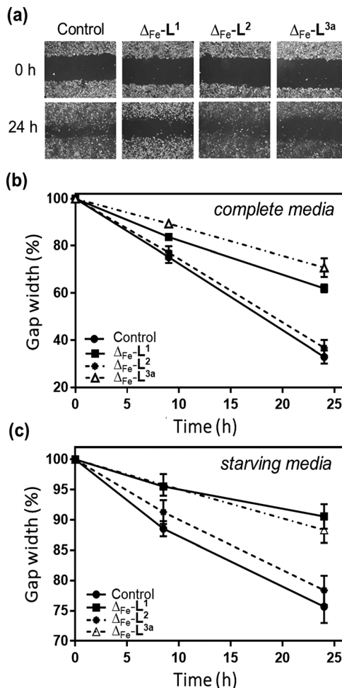
Fig. 8 Wound healing assay of metallohelices. (a) Representative scratch assay images of HCT116 p53 +/+ cancer cells and the effect of treating with metallohelices (at IC 50 concentrations) on scratch closure; images at 0 and 24 h following insertion of a scratch. (b) Quantification of scratch closure at 0, 8.5 and 24 h with cells cultured in complete media (c) a similar result was obtained in starving medium conditions [serum-deprived medium (1% BSA)] indicating that the suppression of wound-healing results at least in part from anti-migration/invasion rather than being due to cell proliferation resulting in closure of the scratch.
