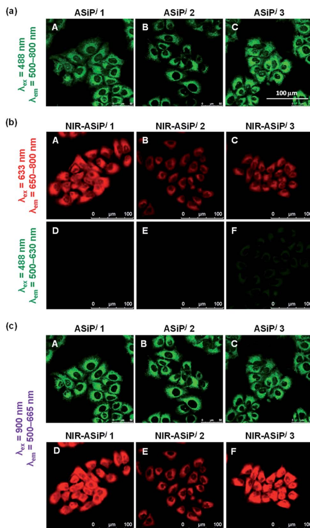
Fig. 4 (a) CLSM images of A549 cells incubated with ASiP i dyes (1.0 \mu M) for 30 min. The images were obtained by excitation at 488 nm and collection of the emissions in the range of 500–800 nm. (b) CLSM images of A549 cells incubated with NIR-ASiP i dyes (10 \mu M) for 30 min. The images were obtained by collecting emissions either from (A–C) the NIR channel (650–800 nm) under excitation at 633 nm or from (D–F) the green channel (500–630 nm) under excitation at 488 nm. (c) TPM images of ASiP i (A–C) and NIR-ASiP i (D–F) dyes. The images were obtained by excitation at 900 nm and collection of the emissions in the range of 500–665 nm. Scale bar: 100 \mu m.
