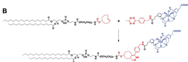
Fig. 4 (A) Radio-HPLC chromatograms of (top) ^{68}\text{Ga} ][Ga]-HBED-CC-tetrazine precursor and (bottom) reaction between 4 and 5, after 15 min at 60 ^{\circ}\text{C} . (B) Scheme of the reaction between TCO-modified PE (4) and ^{68}\text{Ga} ][Ga]-HBED-CC-tetrazine (5).
