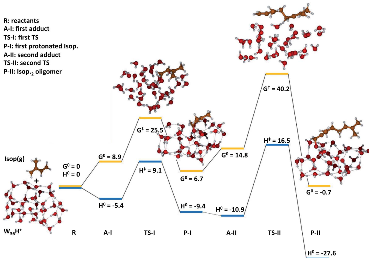
Fig. 6 Quantum mechanics-based free energy and enthalpy landscapes for protonation and oligomerization of isoprene on a cluster consisting of 36 water molecules and an excess proton, (H 2 O) 36 ·H + , representative of very small water droplets. The kinetic barriers preventing proton transfer to isoprene and its subsequent oligomerization were \Delta G^{\ddagger} = 25.5 kcal mol -1 and \Delta G^{\ddagger} = 40.2 kcal mol -1 respectively, which were insurmountable under ambient NTP conditions within the timescale of our experiments (~1 ms). The predictions of this model suggest that the reactions of isoprene in electrosprays cannot involve liquid-phase drops. These predictions also support the proposed mechanisms M 3 by ruling out the possible reactions through M 2 .
