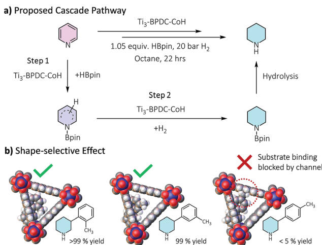
Fig. 4 (a) Proposed cascade reduction pathway. (b) Shape selectivity of the cascade reduction of 3-( m/p/o -tolyl)pyridine.
