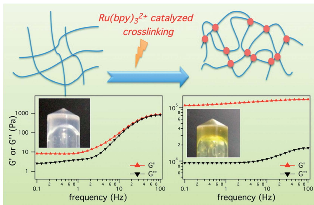
Fig. 4 \text{Ru}(\text{bpy})_3^{2+} catalyzed photo crosslinking to enhance the mechanical stability of the peptide-based hydrogels. 66
