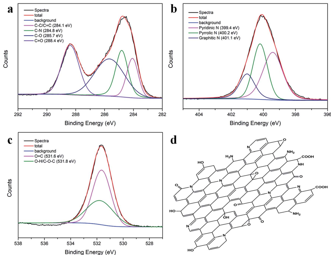
Fig. 3 XPS spectra of the (a) C 1s , (b) N 1s and (c) O 1s of N-CDs. Spectra represented the measured spectra, the total was the fitted curve, background meant the baseline of the measured spectra, and other spectra were obtained by deconvoluting the corresponding spectra. (d) The probable molecular structure of the N-CDs.
