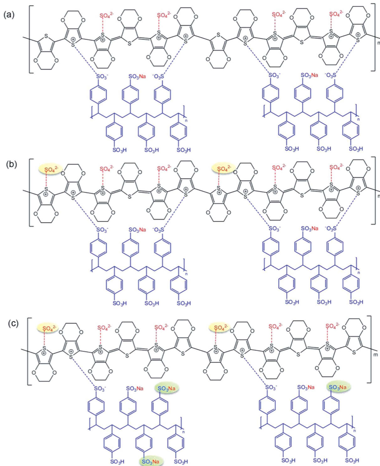
Scheme 3 Proposed structure of PEDOT:PSS at the EDOT : PSS weight ratio of 1 : 11 and at various EDOT : \text{Na}_2\text{S}_2\text{O}_8 mole ratios: at an EDOT : \text{Na}_2\text{S}_2\text{O}_8 mole ratio (a) lower than 1 : 2, (b) 1 : 2, where \text{SO}_4^{2-} acts as a secondary dopant and (c) higher than 1 : 2, where a higher PSSNa amount is generated.
