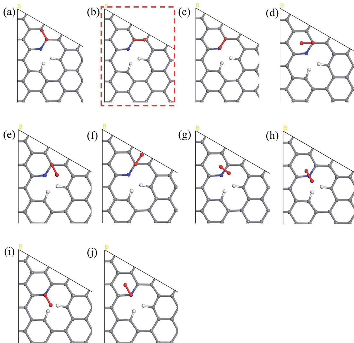
Fig. 2 The potential sites where O_2 can be located on the N6 substrate for the first step of the ORR. N6_S1_(a) CBC1 (b) CBC2 (c) CBN (d) CH1 (e) CH2 (f) CH3 (g) HBH (h) HNH (i) NH1 and (j) NH 2 . The model marked by red dashed line has the lowest energy upon geometry optimization, indicating the most likely adsorption configuration and is used in the free energy diagram.
