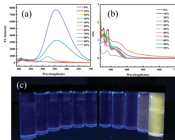
Fig. 2 (a) Fluorescence spectra and (b) absorption spectra in different THF/water (v/v) mixtures. (c) Optical images of ODFRPTZ in the mixed solution (20 μM, λ ex = 365 nm).
