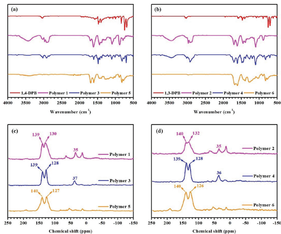
Fig. 1 FT-IR spectrum of (a) 1,4-DPB and 1,4-DPB-based polymer materials, and (b) 1,3-DPB and 1,3-DPB-based polymer materials; solid state cross-polarization (CP) 13 C MAS natural abundance NMR spectrum of (c) 1,4-DPB-based polymer materials, and (d) 1,3-DPB-based polymer materials.
