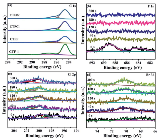
Fig. 3 (a) C 1s XPS spectra of CTF-1 and CTFX samples. (b) F 1s XPS spectra of CTFF, (c) Cl 2p XPS spectra of CTFCl and (d) Br 3d XPS spectra of CTFBr after \text{Ar}^+ sputtering from 0 to 300 s.
