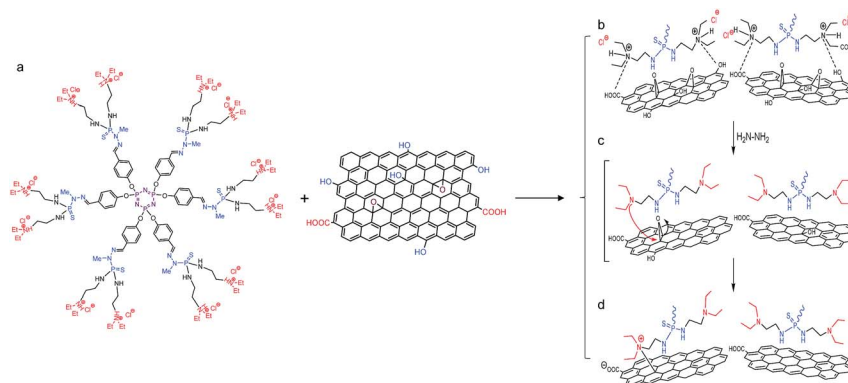
Scheme 1 Chemical interplay occurring at the dendrimer–graphene oxide interface. (a) Typical chemical structure of the first generation phosphorus dendrimer \text{DG}_1 and oxygenated graphene oxide sheets. (b) Plausible mechanism occurring during interfacial complexation of ternary diethyl- N -amino-ammonium chloride arms and (c and d) the subsequent chemical reduction. See S10 in the ESI† for further discussion.
