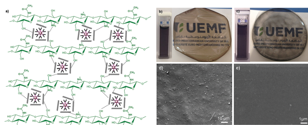
Fig. 6 (a) Intercalation of \text{DG}_n\text{-RGO} within the fibrillary network of chitosan. (b) Aqueous dispersion of \text{DG}_4\text{-GO} and the resulting transparent \text{CS@DG}_4\text{-GO} film (top) and (d) the corresponding SEM analysis. (c) Aqueous dispersion of \text{DG}_4\text{-RGO} and the resulting transparent \text{CS@DG}_4\text{-RGO} film (top) and (e) the corresponding SEM analysis.
