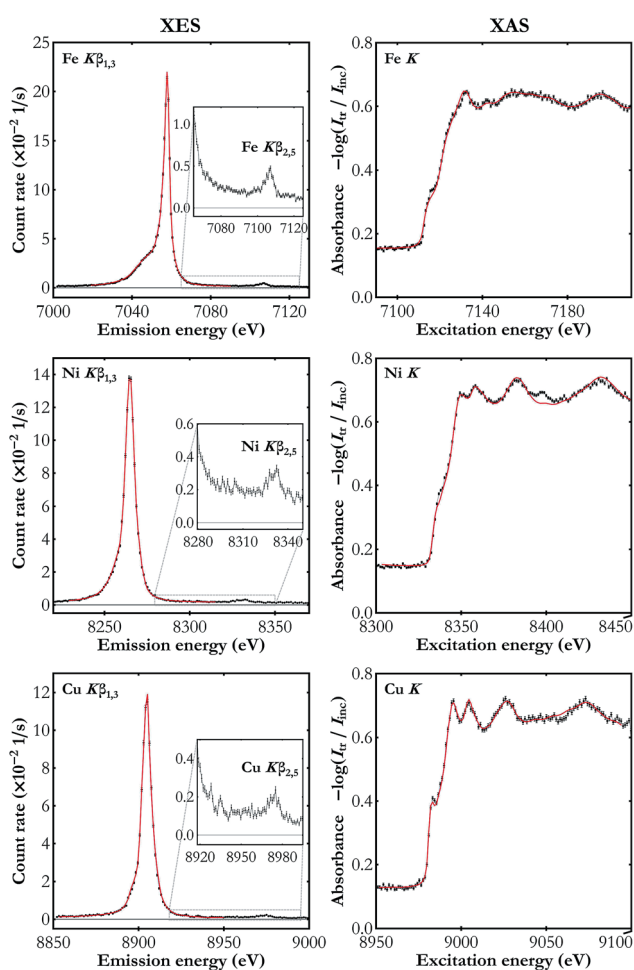
Fig. 4 The simultaneously measured K \beta XES (left-hand side) and K-edge XAS spectra (right-hand side) for Fe, Ni and Cu foils (black dots). The reference spectra used in the energy calibration are also shown (red line). 40–44 The valence-to-core emission lines are enlarged in the insets. The XAS spectra plots show the absorbance calculated using the transmitted and the incident beam spectra I_{tr} and I_{inc} , respectively. The statistical uncertainty does not exceed 0.003 \text{ s}^{-1} \text{ eV}^{-1} and 0.008 \text{ eV}^{-1} in all the presented XES and XAS spectra, respectively.
