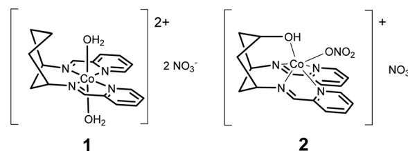
Scheme 1 Catalysts 1 and 2 .
