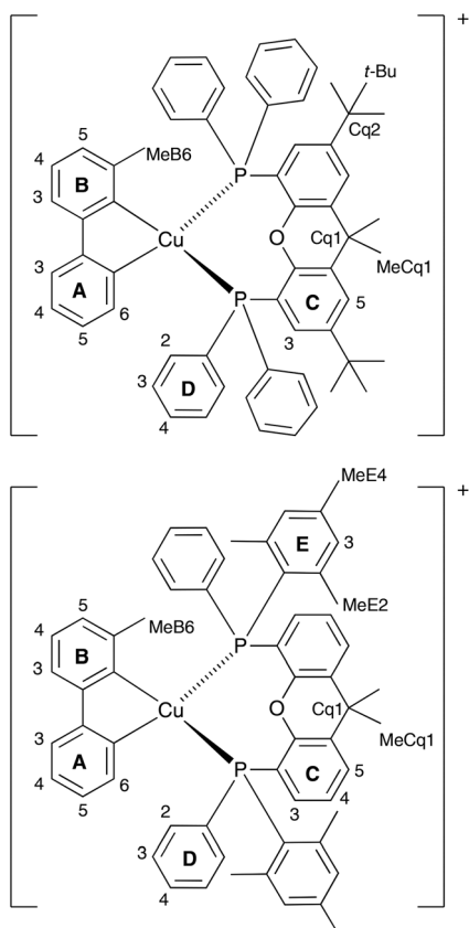
Scheme 3 Structures of [\text{Cu}^{\text{I}}(\text{Bu}_2\text{xantphos})(6\text{-Mebpy})]^+ and [\text{Cu}(\text{xantphosMes}_2)(6\text{-Mebpy})]^+ with labelling for NMR spectroscopic assignments.
