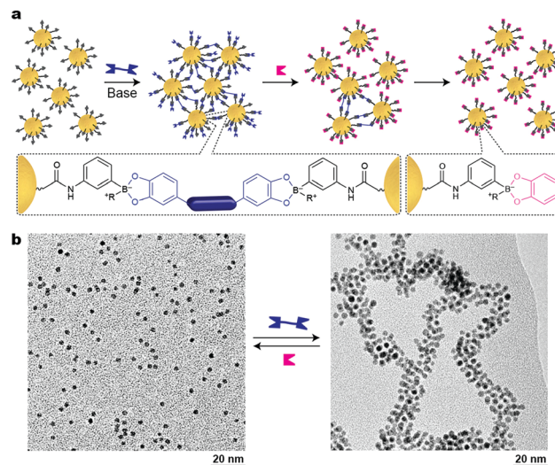
Fig. 7 Nanoparticle aggregation driven by dynamic covalent chemistry. (a) NP assembly followed by disassembly induced by a ditopic and a mono-topic boronic acid, respectively. (b) TEM images of free and covalently assembled Au NPs. Adapted with permission from ref. 45 (copyright 2016, Royal Society of Chemistry).
