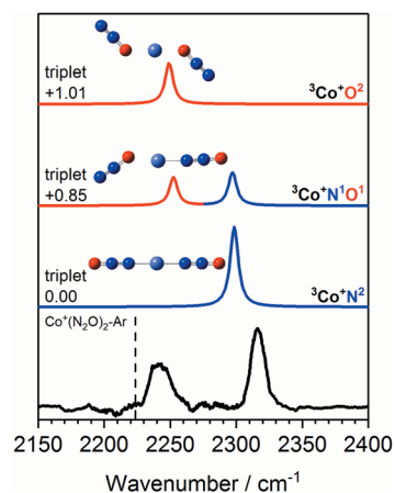
Fig. 5 Experimental IRPD spectrum of the Co^+(N_2O)_2-Ar complex along with simulated IR spectra of low-lying isomers of the ground triplet state in the region of the N_2O asymmetric ( N=N ) stretch. Simulated IR bands corresponding to N-bound and O-bound ligands are indicated in blue and red, respectively. The relative energies of different isomers are given in eV. The vertical dashed line indicates the wavenumber of the \nu_3(N=N) mode in isolated N_2O at 2223.5\text{ cm}^{-1} . 51
