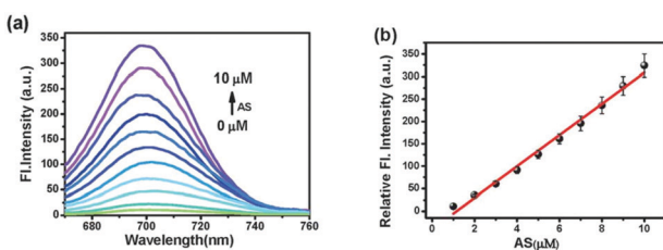
Fig. 107 (a) Fluorescence responses of 65 ( 2 \mu\text{M} ) to different concentrations of Angel's salt (AS) with emission ranging from 670 to 760 nm. \lambda_{\text{ex}} = 690 \text{ nm} . (b) Relationship between the relative fluorescence intensity at 700 nm and concentrations of AS (0, 1, 2, 3, 4, 5, 6, 7, 8, 9, 10 \mu\text{M} ). Fluorescence spectra were acquired in HEPES buffer solution (10 mM, 0.5% DMSO, 0.5% TW 80, pH 5.0). Copyright 2014 Royal Society of Chemistry.
