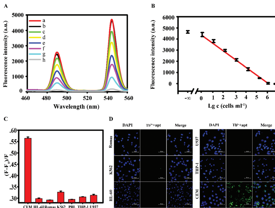
Fig. 3 (A) Fluorescence emission spectra of the Tb^{3+} -apt fluorescent aptasensor in the presence of different concentrations of CCRF-CEM cells (a. Tb^{3+} -apt, b. 10^0 cells per 200 \mu l, c. 10^1 cells per 200 \mu l, d. 10^2 cells per 200 \mu l, e. 10^3 cells per 200 \mu l, f. 10^4 cells per 200 \mu l, g. 10^5 cells per 200 \mu l, h. 10^6 cells per 200 \mu l). (B) Linear relationship between the fluorescence intensity and the concentration of CCRF-CEM cells. (C) Specificity of the fluorescent aptasensor for CEM. The fluorescence intensity rate (F - F_0)/F_0 of the Tb^{3+} -apt fluorescent aptasensor in the presence of CEM, HL-60, Ramos, K562, PBL, THP-1, and U937 cells, respectively ( 1 \times 10^6 cells per 200 \mu l), where F and F_0 are the fluorescence intensity without and with detection cells at 545 nm. Excitation: 290 nm. (D) Fluorescence micrographs of six different cells after mixing with Tb^{3+} -apt. Nuclei were stained with DAPI. Scale bars indicate 50 \mu m.
