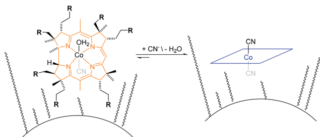
Fig. 1 Schematic overview of cyanide binding with immobilized corrinoids in the detection zone of the CyanoKit. R = \text{COOC}_n\text{H}_{2n+1} where n = \{1,4\} .
