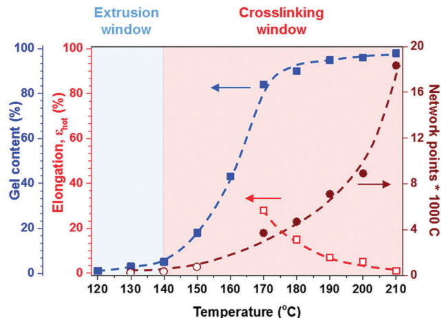
Fig. 5 Effect of temperature on hot set elongation ( \square ), number of network points per 1000 C atoms ( \bullet from hot set, \circ from rheology), and gel content ( \blacksquare ) for a 1.7:1 stoichiometric p(E-stat-GMA):p(E-stat-AA) blend cross-linked for 5 minutes; note that industrial standards for electrical insulation demand a hot set elongation of \epsilon_{\text{hot}} = \lambda_{\text{hot}} - 100\% < 75\% for \sigma = 0.2 \text{ MPa} . 42
