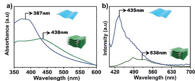
Fig. 4 UV-vis (a) and emission (b) spectra of bulk TTA-DFP COFs (green line) and exfoliated TTA-DFP CONs (blue line) dispersed in water at room temperature, \lambda_{\text{ex}} = 375 \text{ nm} .
