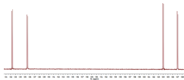
Fig. 3 NMR spectra for [PF 2 (BIMeEt 3 )] 3+ in CD 3 CN.
