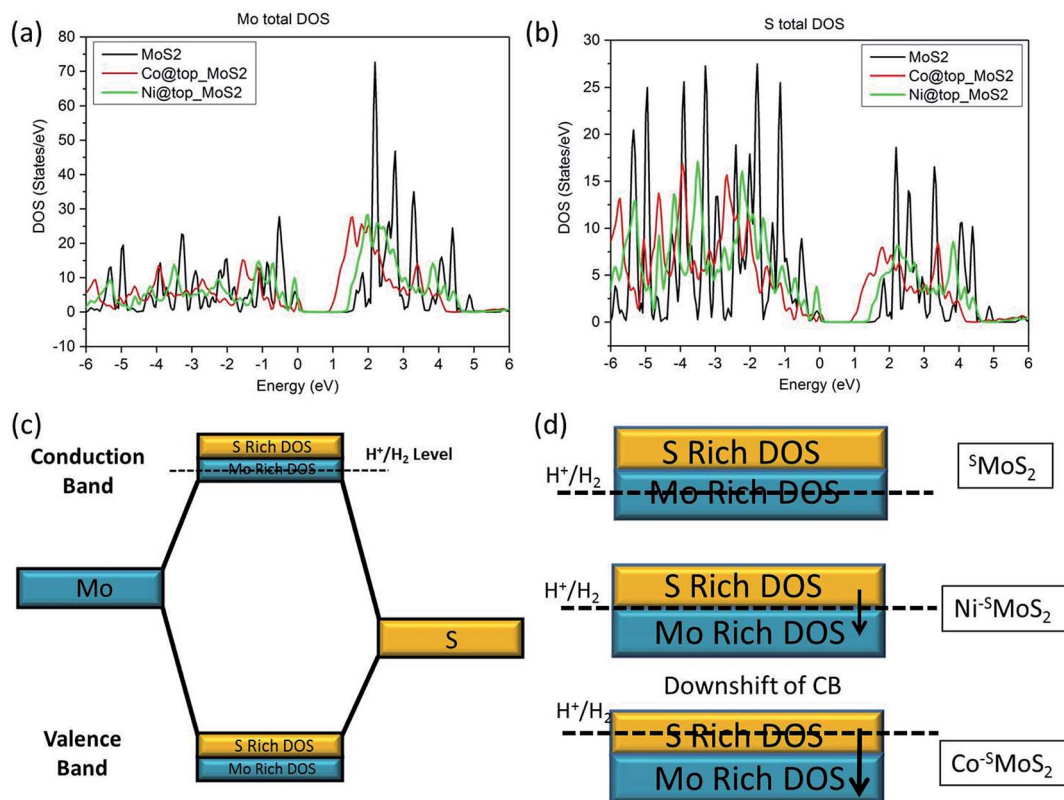
Fig. 7 Calculated Density of States (DoS) of (a) Mo and (b) S in ^s\text{MoS}_2 , \text{Co-}^s\text{MoS}_2 and \text{Ni-}^s\text{MoS}_2 (c) simplified molecular orbital diagram of \text{MoS}_2 (d) downshift of the conduction band (CB) upon addition of a single Co and Ni metal atom at the Mo atop site, respectively.
