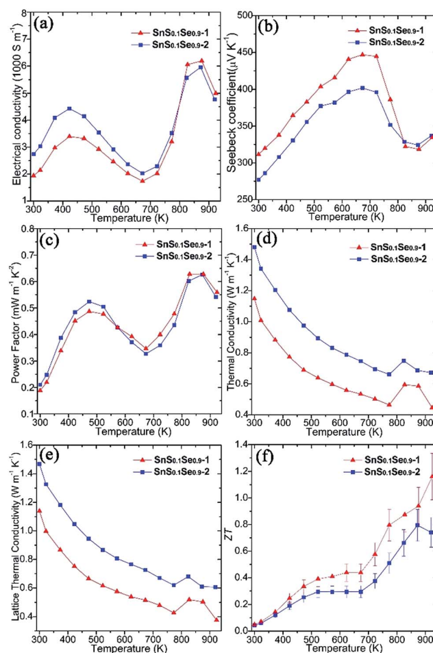
Fig. 5 Thermoelectric properties of \text{Sn}_{0.1}\text{Se}_{0.9} pellets \text{Sn}_{0.1}\text{Se}_{0.9-1} and \text{Sn}_{0.1}\text{Se}_{0.9-2} measured perpendicular to the pressing direction: (a) the electrical conductivity ( \sigma ), (b) the Seebeck coefficient ( S ), (c) the power factor ( S^2\sigma ), (d) the thermal conductivity ( \kappa ), (e) the lattice \kappa ( \kappa_L ), and (f) ZT as a function of temperature.
