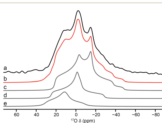
Fig. 7 (a) ^{17}\text{O} (14.1 T, 20 kHz) MAS NMR spectrum of calcined Al, Ga (50 : 50) MIL-53 (hydroxyl region only). Overall fit (b) and deconvolution into components resulting from hydroxyls that bridge between (c) Al/Al, (d) Al/Ga and (e) Ga/Ga.
