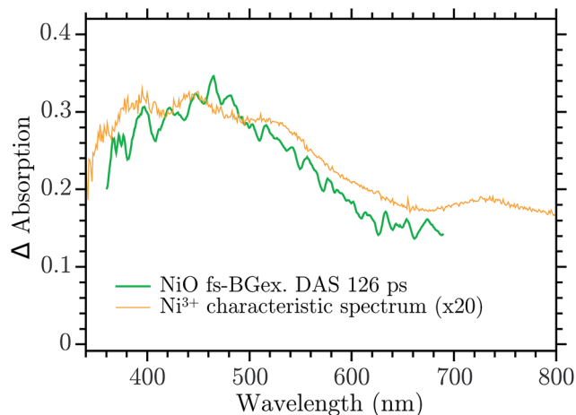
Fig. 7 Comparison between the 126 ps component of the DAS in the \text{Ni}^{3+} characteristic spectrum found in ref. 24.
