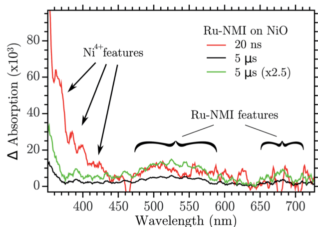
Fig. 9 Transient absorption of Ru-NMI sensitized on NiO and excited at 460 nm. The green trace is the 5 \mu\text{s} trace normalized to the 20 ns one at 500 nm.
