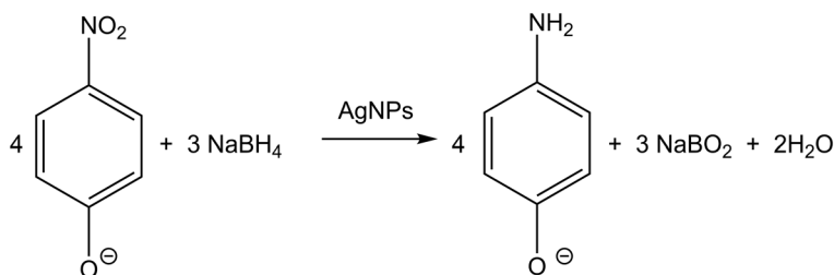
Fig. 11 Reduction of 4-NP to 4-AP by excess NaBH 4 . Conditions: 3.3 \times 10^{-5} M 4-NP and 6.6 \times 10^{-2} M NaBH 4 at room temperature.
